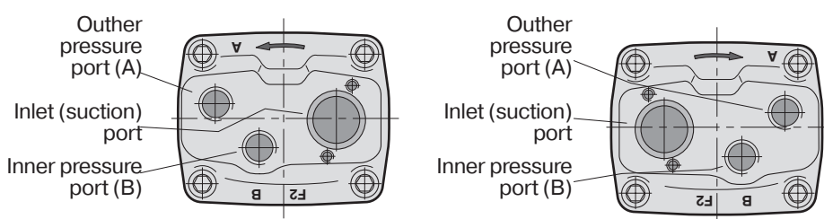
End cap for right hand rotating pump End cap for left hand rotating pump
