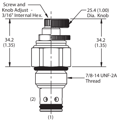
Screw/Knob Version
