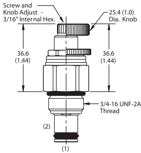
Screw/Knob Version
