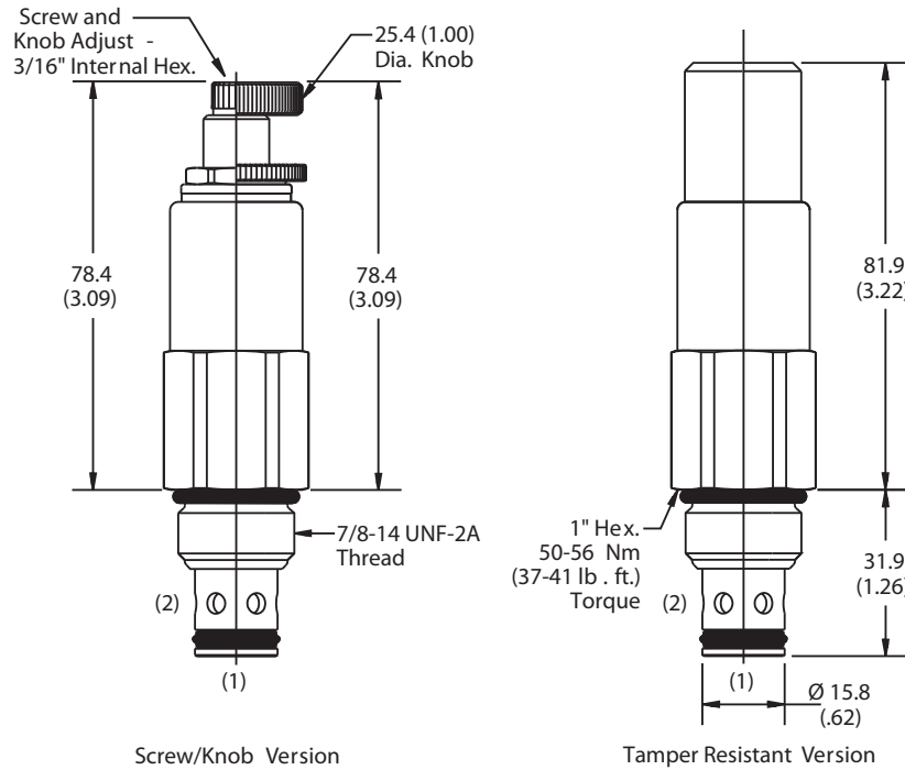
Screw/Knob Version
