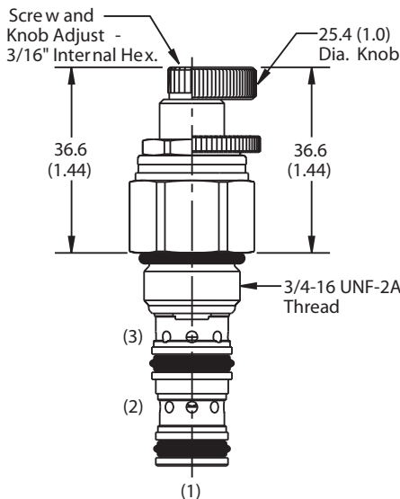
Screw/Knob Version
